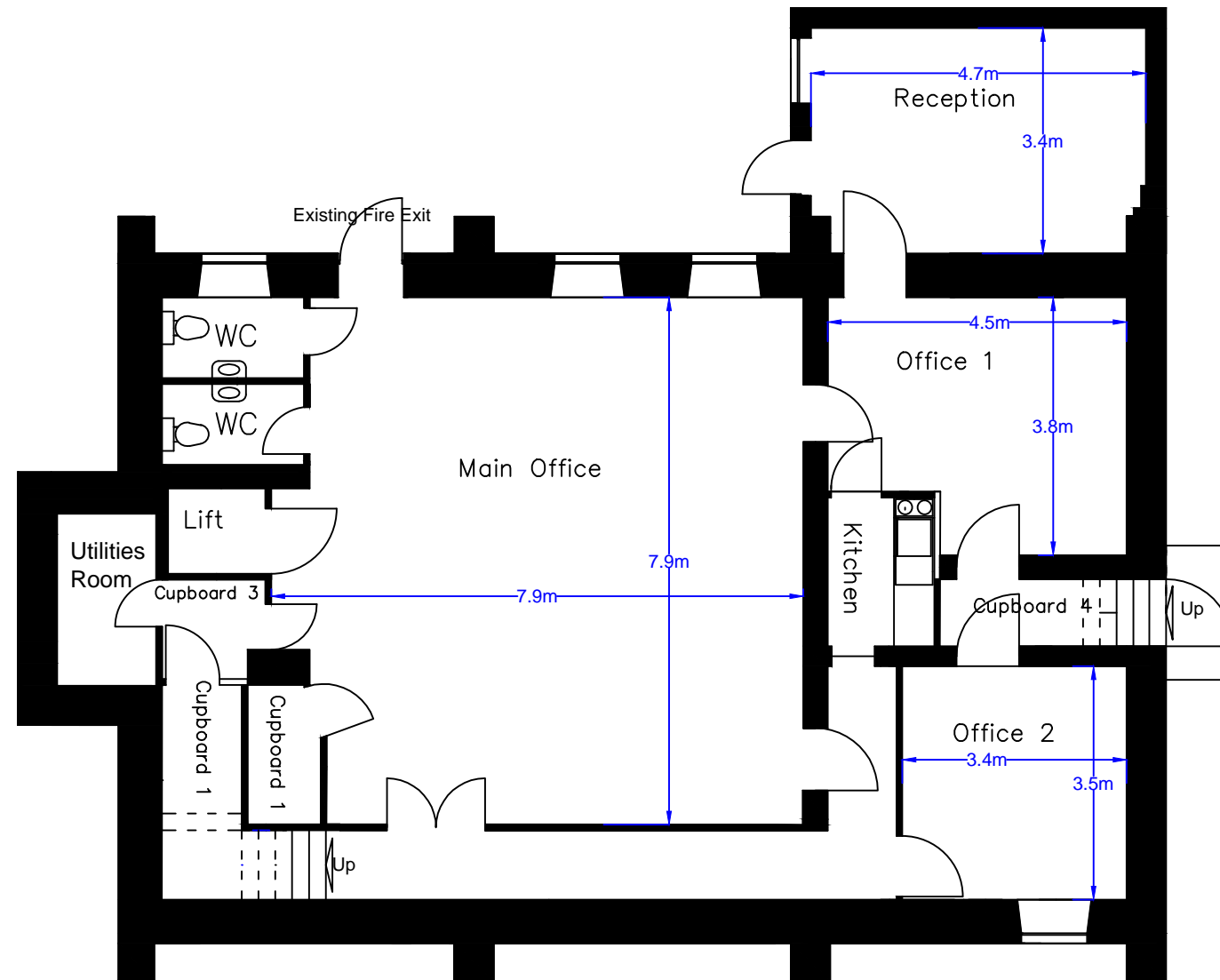
8DT12: 8 Derby Terrace Lower Ground Floor Plan as Proposed Page 1 of 1, Scale 1:100 at A3
